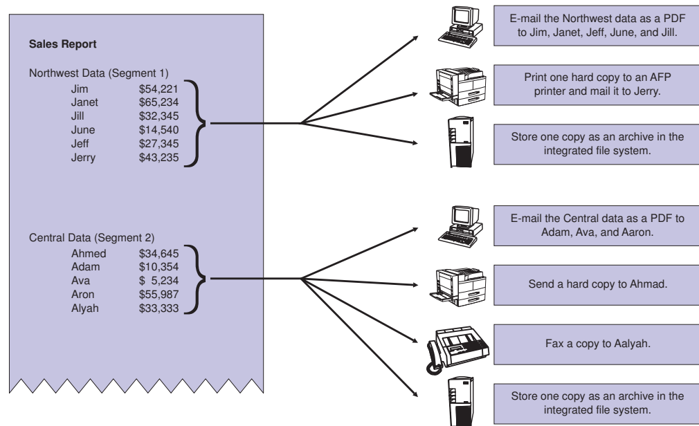
Figure 14. Routing Tags
