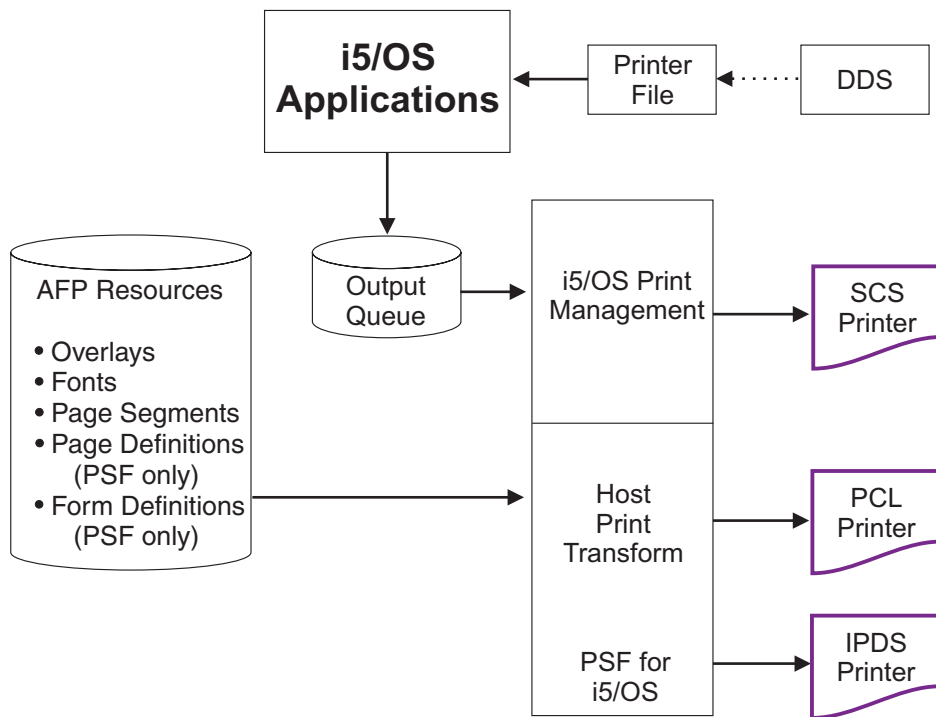
Figure 2. iSeries Printing without Infoprint Server
