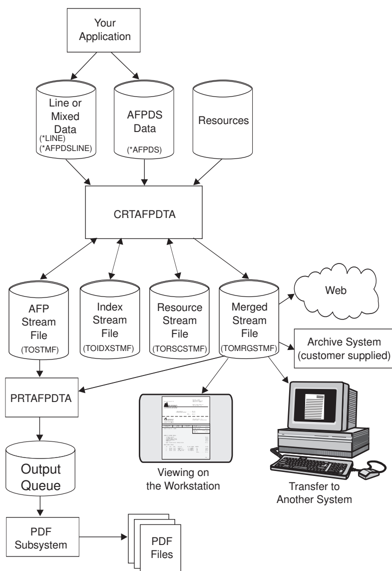
Figure 5. Using CRTAFPDTA
